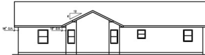
REAR ELEVATION SCALE -- 1/8"=1'-0"
